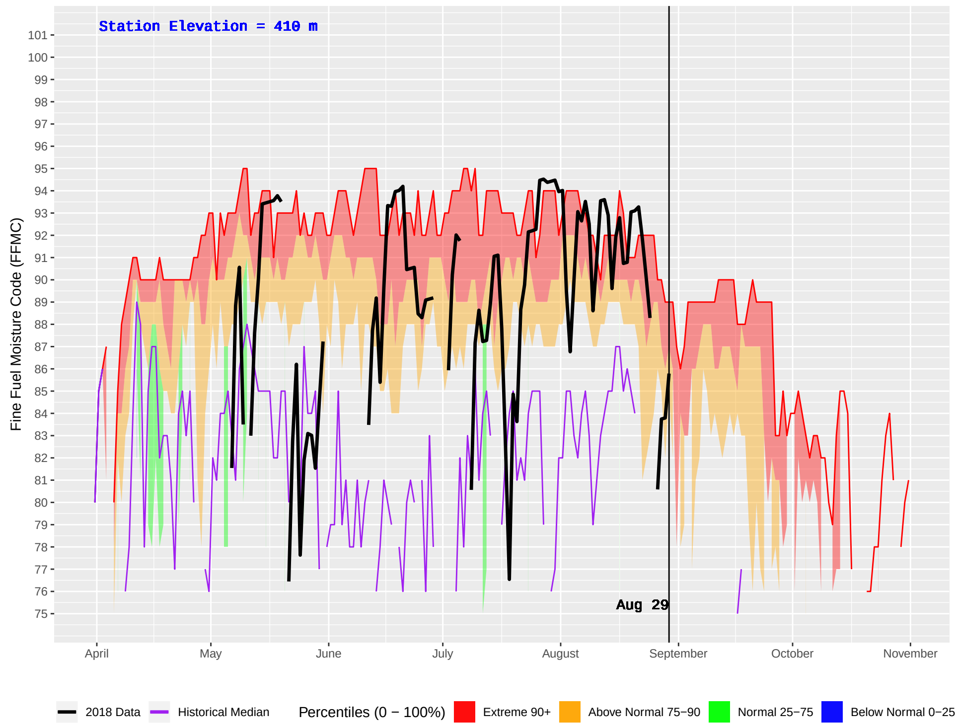
UPPER KISPIOX (431) : Historical (1986–2016) and Current (2018) Daily Fine Fuel Moisture Code (FFMC)
