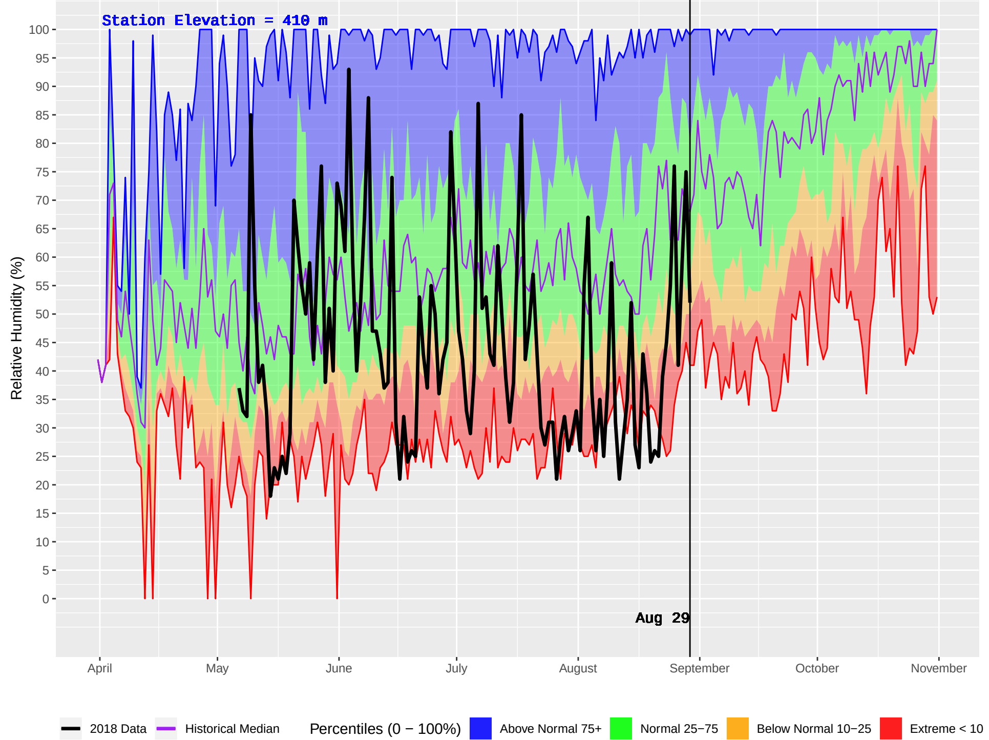
UPPER KISPIOX (431) : Historical (1986–2016) and Current (2018) Daily Relative Humidity
