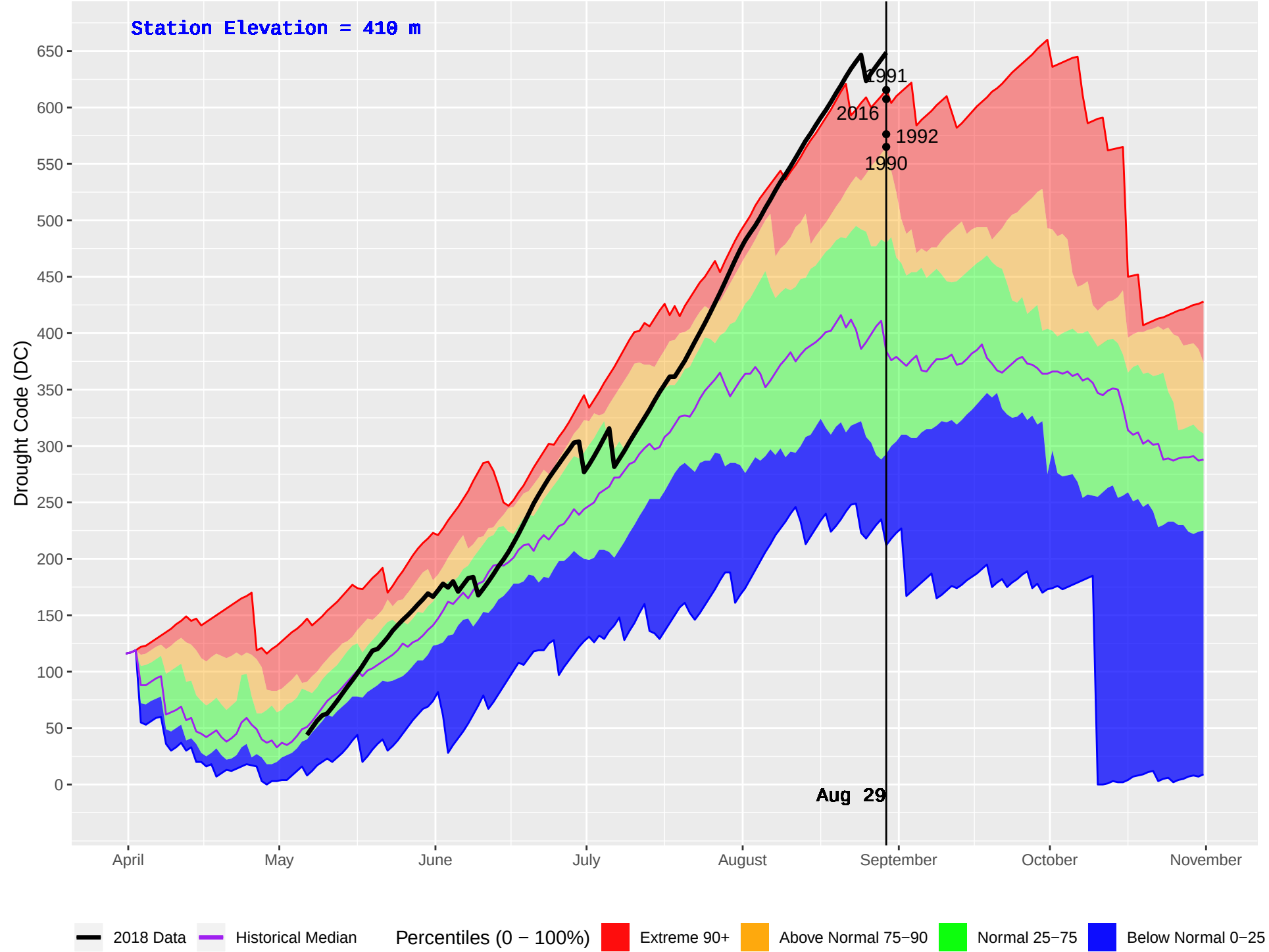
UPPER KISPIOX (431) : Historical (1986–2016) and Current (2018) Daily Drought Code (DC)
