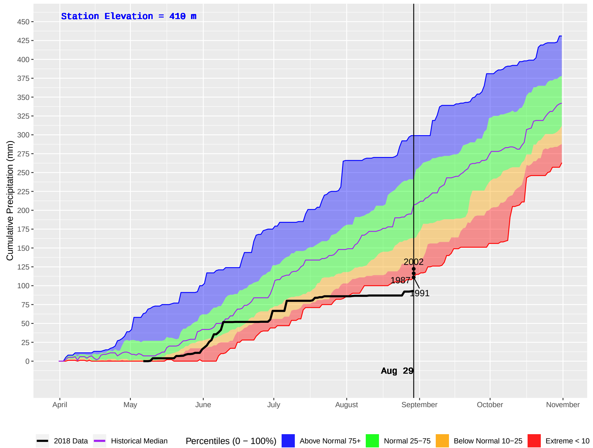
UPPER KISPLOX (431) : Historical (1986–2016) and Current (2018) Daily Cumulative Precipitation
