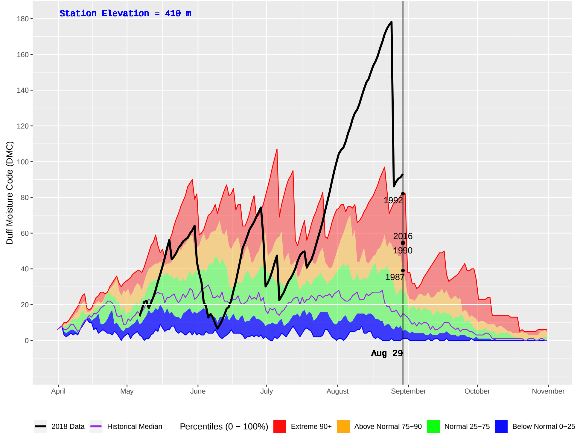
UPPER KISPIOX (431) : Historical (1986–2016) and Current (2018) Daily Duff Moisture Code (DMC)
