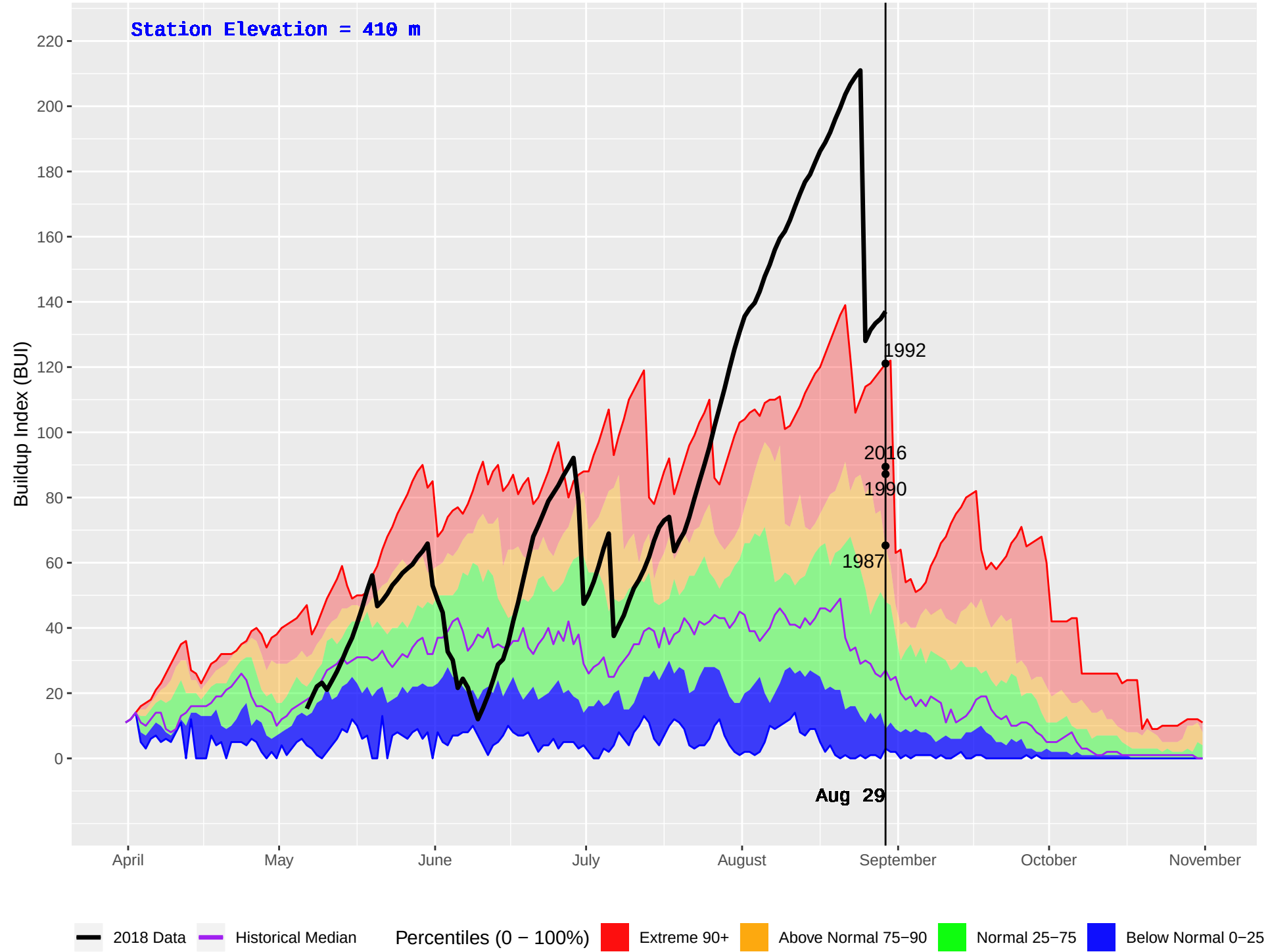
UPPER KISPIOX (431) : Historical (1986–2016) and Current (2018) Daily Buildup Index (BUI)
